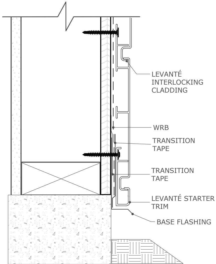
SECTION VIEW
