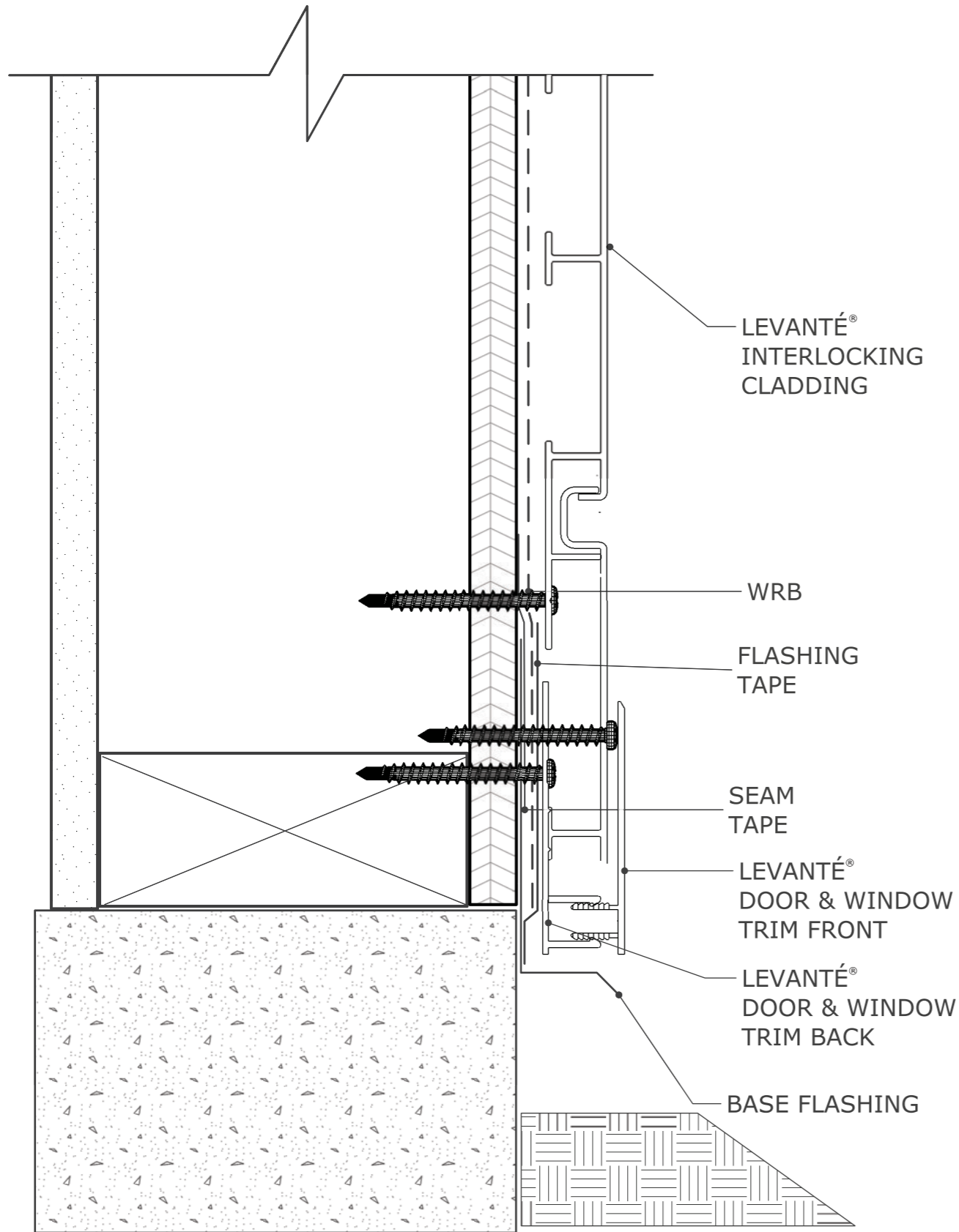
SECTION VIEW
