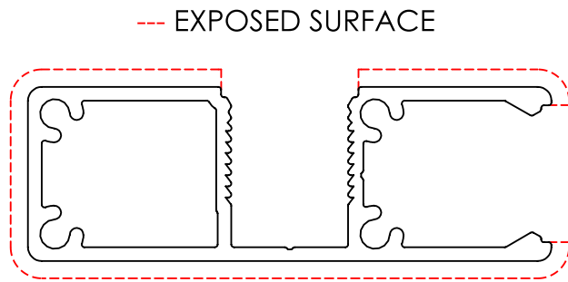
EXTRUSION PROFILE SCALE 1:1
