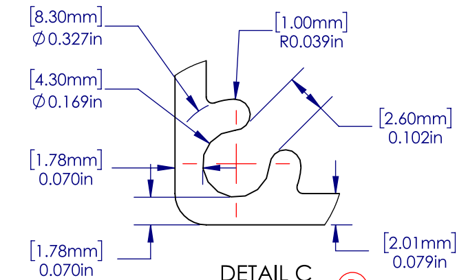
DETAIL C SCALE 3:1
