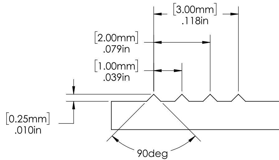
DETAIL ID MARKS SCALE 12:1
