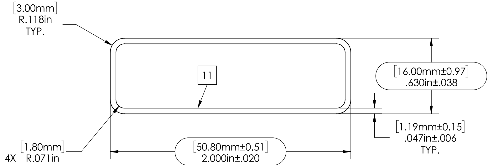
EXTRUSION PROFILE SCALE 2:1
