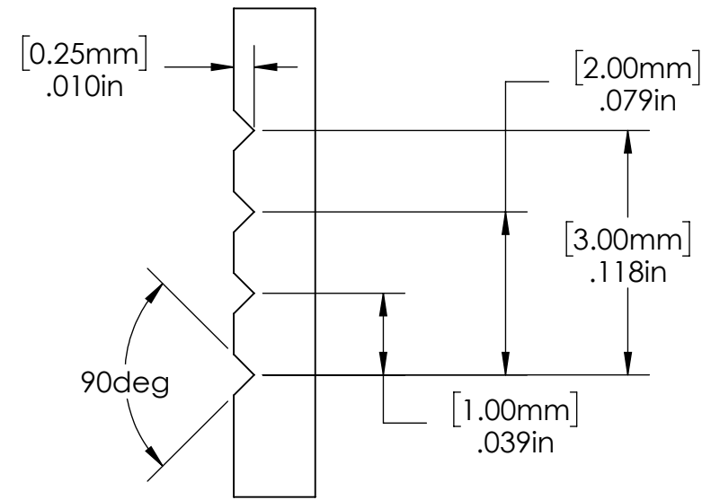
DETAIL ID MARKS SCALE 12:1
